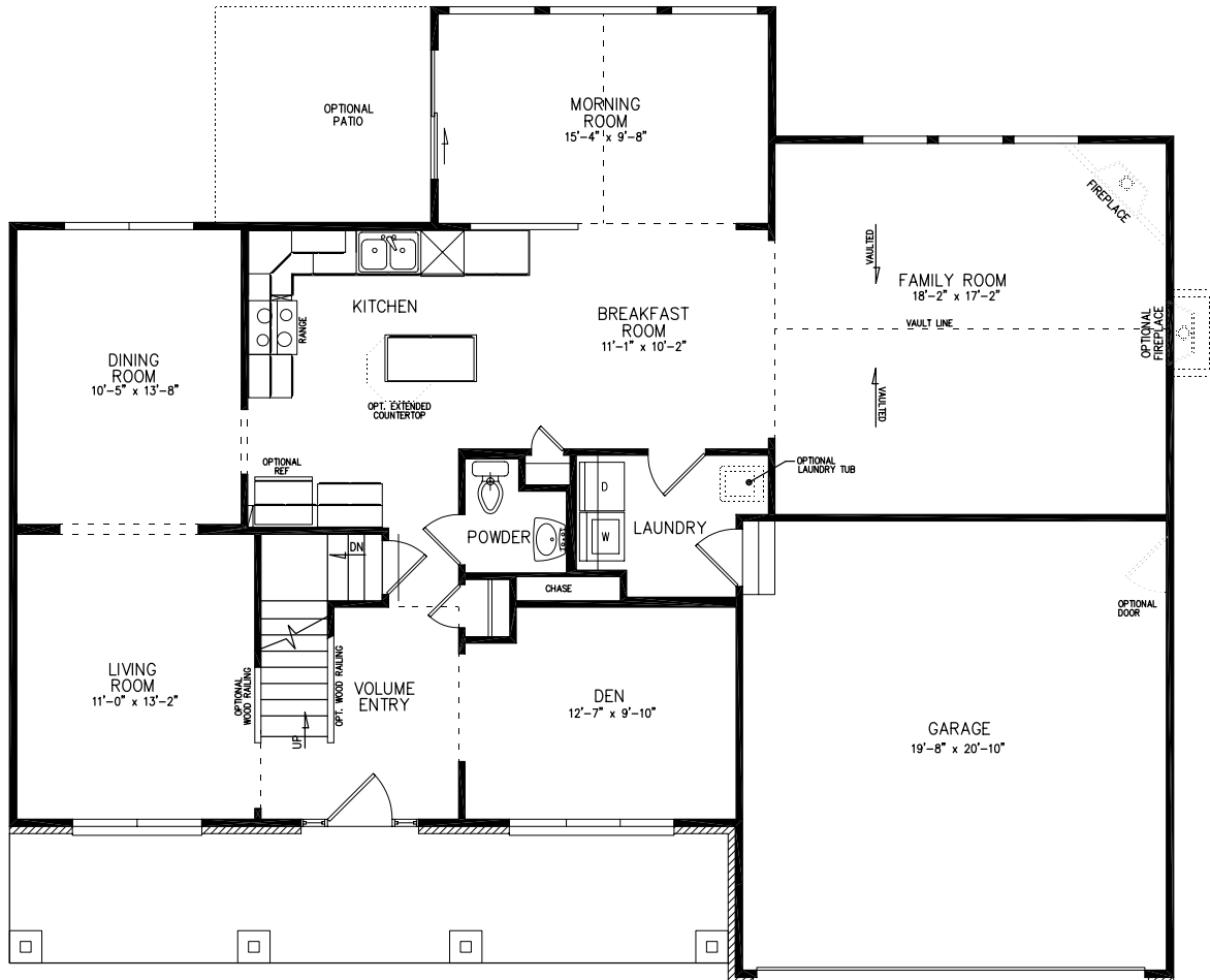
First Floor
