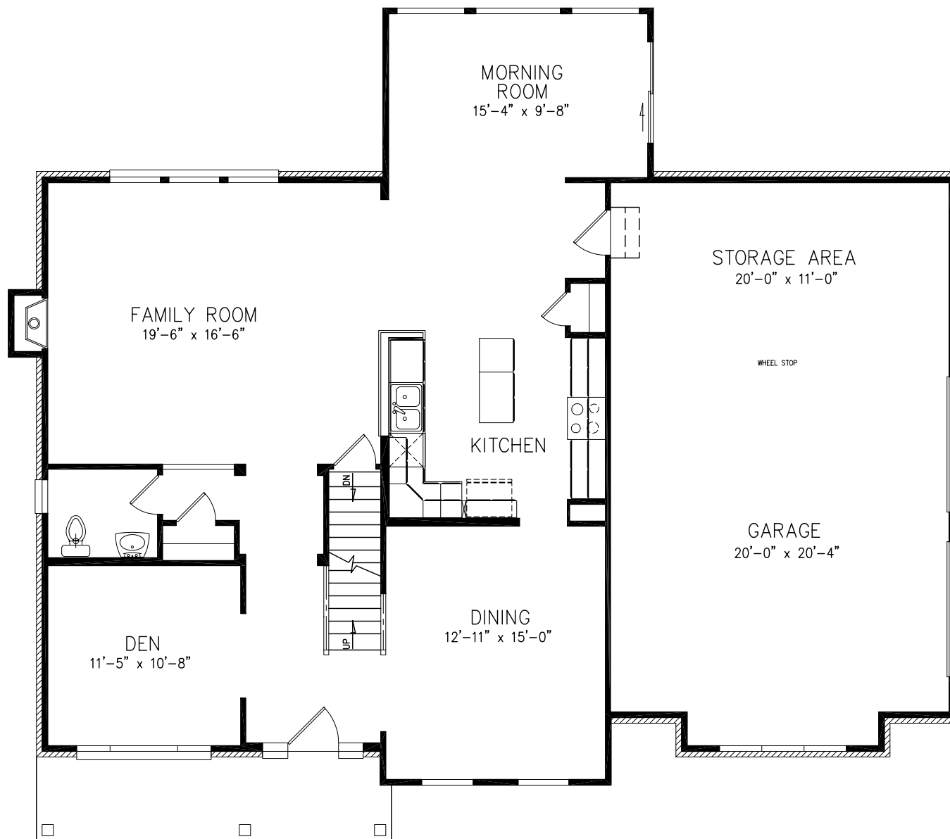
1ST FLOOR EXTENDED PLAN
