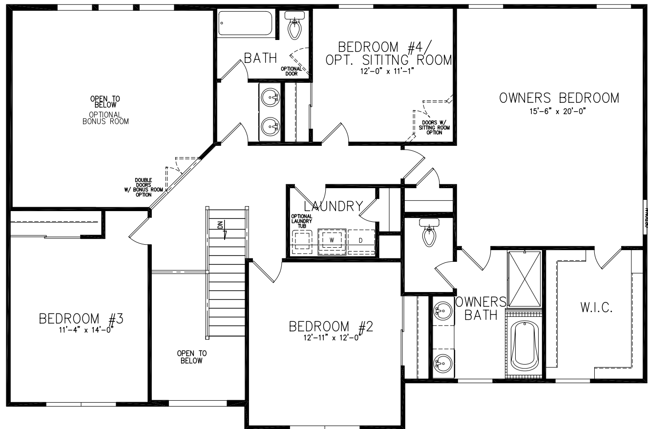
2ND FLOOR PLAN #1
