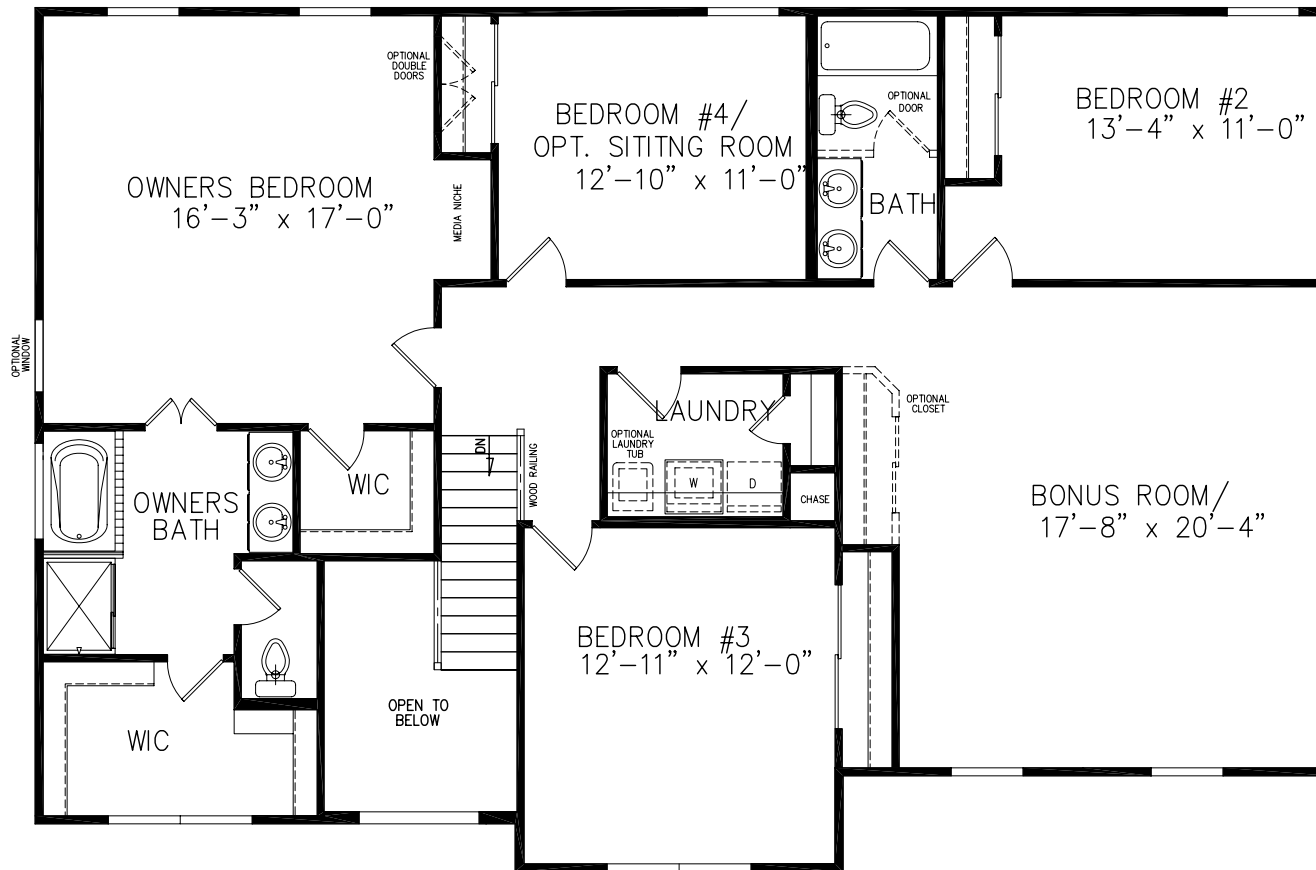
2ND FLOOR PLAN #2
