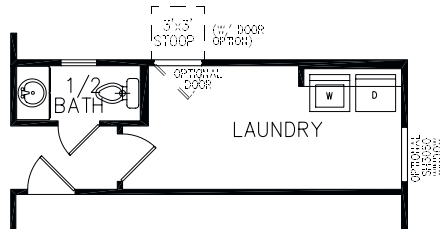
EXTENDED LAUNDRY ROOM OPTION
