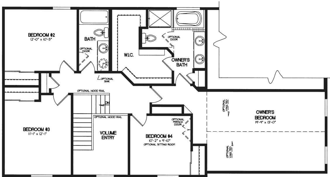
Second Floor
