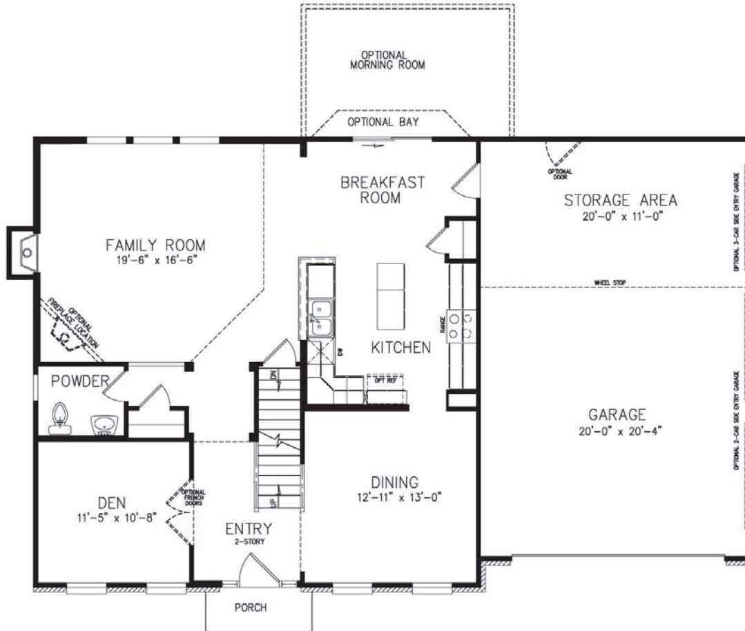
Floor plan shown with elevation A
