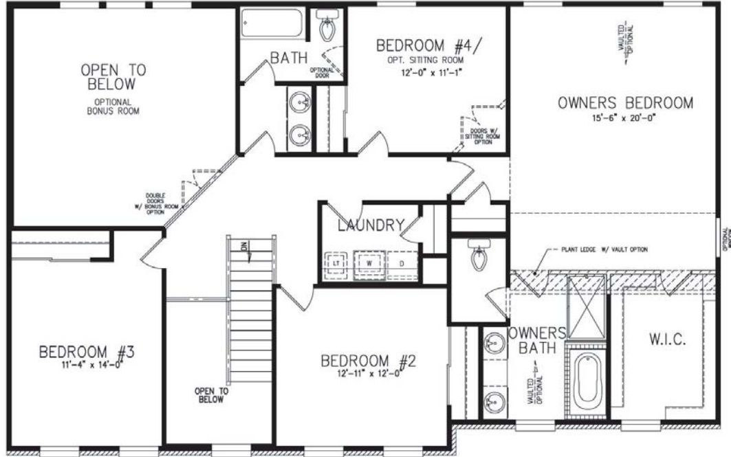
Second Floor
