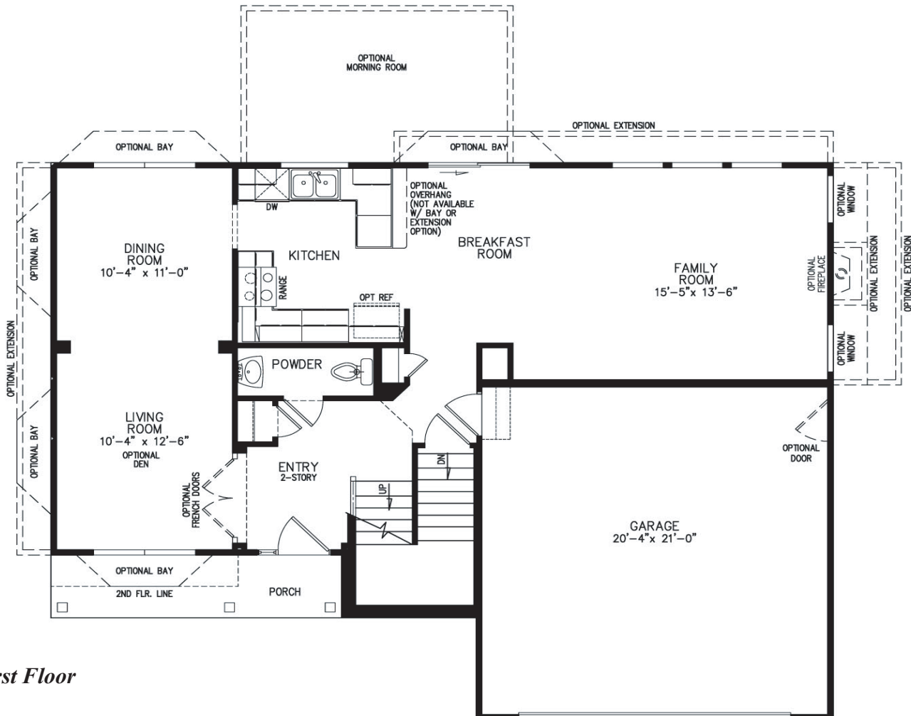
Floor plan shown with elevation A
