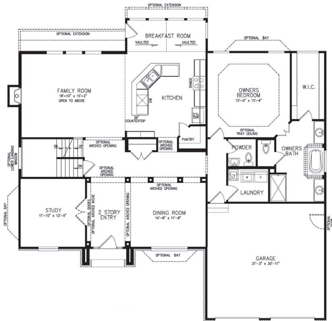
Floor plan shown with elevation A
